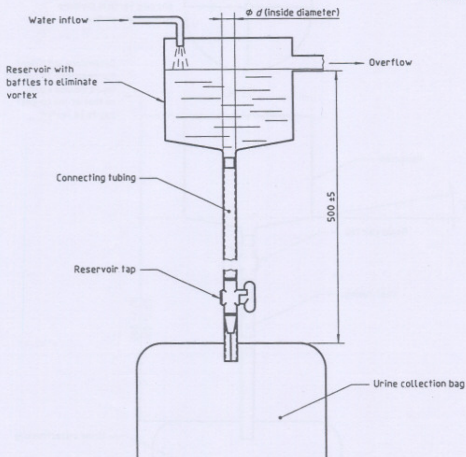
Figure 1 — Filling system for determination of test volume
